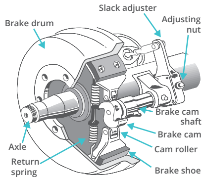
Figure 12. S-cam brake assembly
