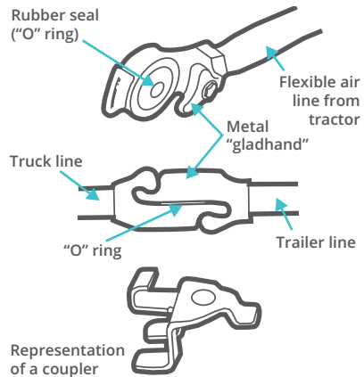
Figure 40. Gladhands
