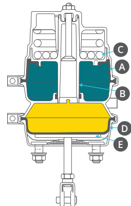
Figure 33. Spring brakes
